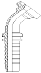
Two Piece Crimp Code 61 Flange Page 121
