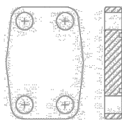
Code 61 Flange Blanking Plate Page 130
