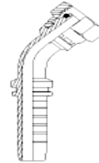
Two Piece Crimp Metric Light Female Page 122
