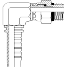
Two Piece Crimp UNO Male Swivel Page 123
