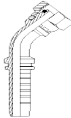
Two Piece Crimp Metric Heavy Female Page 122
